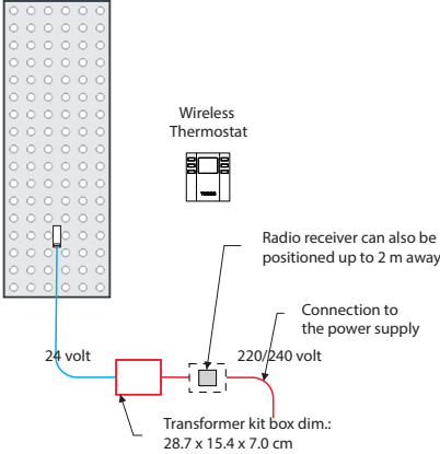
Connection via wall-mounted Wireless Thermostat (ZRF007)
