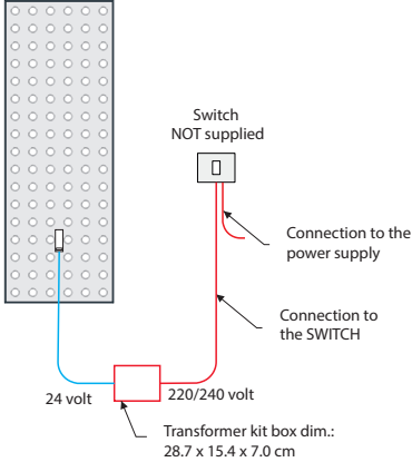
Direct connection to a switch (not supplied) or to a home automation system
