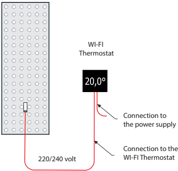
Connection via wall-mounted WI-FI Thermostat «ZRF» (ZRF081 - ZRF082)
