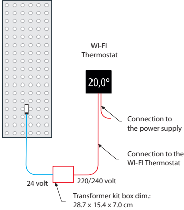
Connection via wall-mounted WI-FI Thermostat «ZRF» (ZRF081 - ZRF082)
