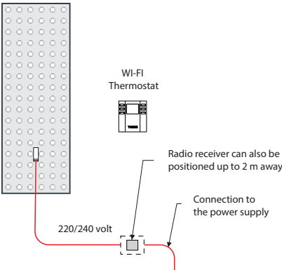
Connection via wall-mounted Wireless Thermostat (ZRF007)
