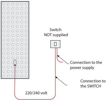
Direct connection to a switch (not supplied) or to a home automation system
