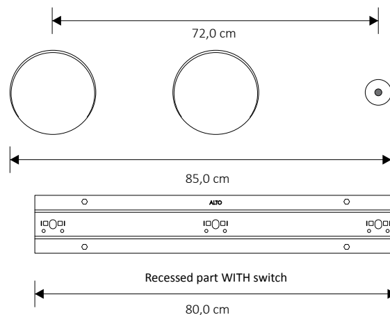
Version WITH switch
