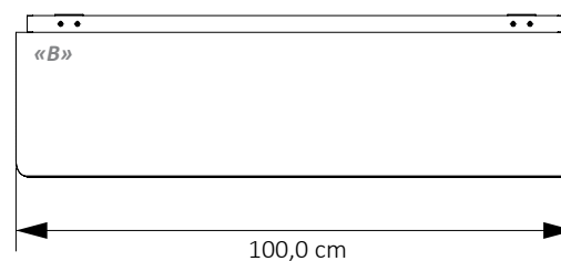
JJ24#100 Without towel rail
