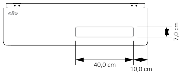
JJ24_CD#100 Towel rail - Closed on the Right
