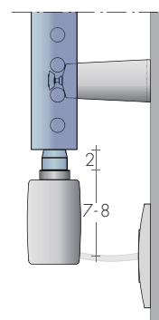
Art. R...IIF ø1/2", with Faston for Digital Thermostat
